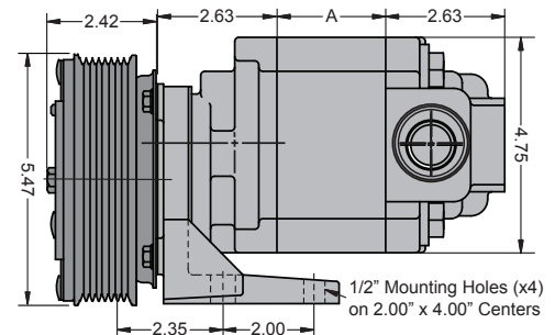
Clutch Pump 8 Groove Serpentine
